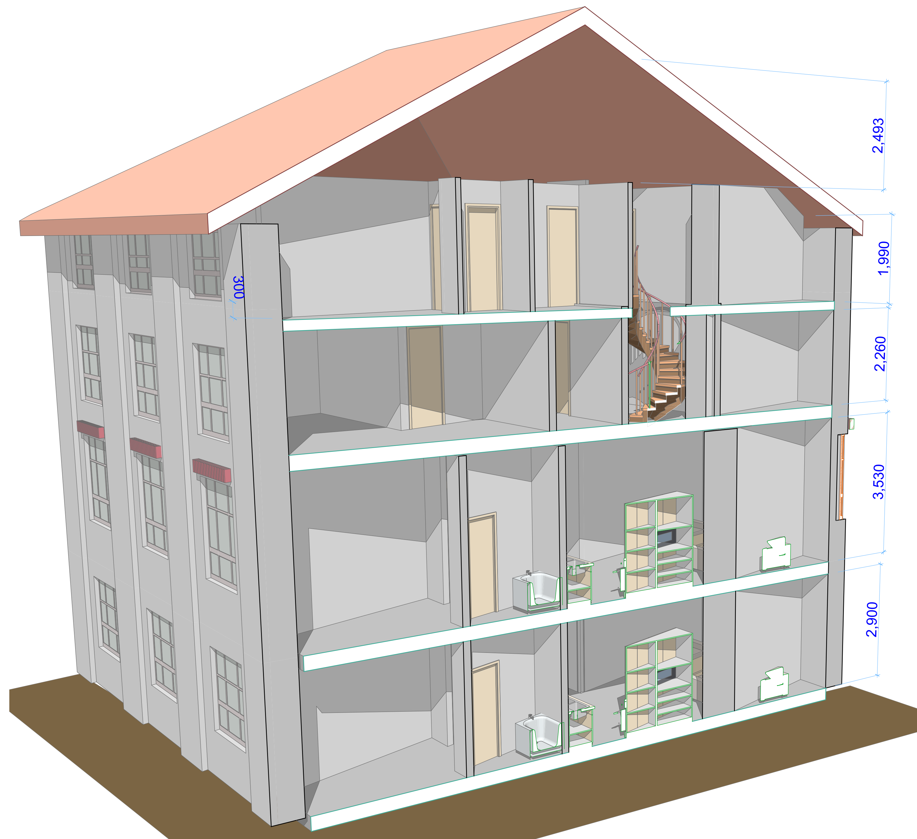
Floor Elevations
